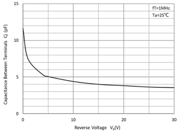
Fig 2: Capacitance Capability
